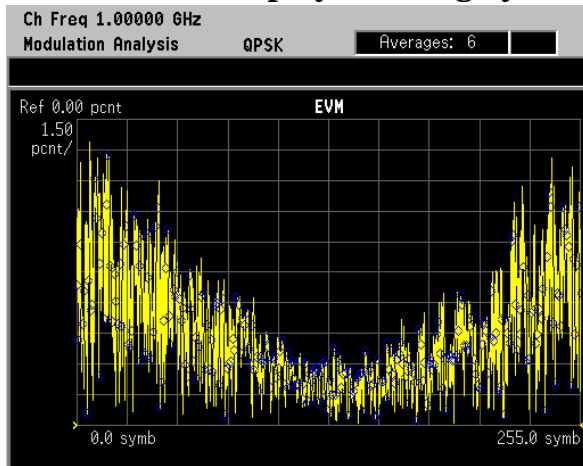
EVM vs Time Display Showing Symbol Rate Error
