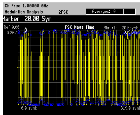
Figure 2-41 FSK Measured Time
