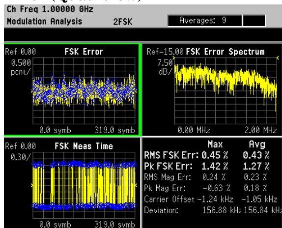
Figure 2-34 FSK Error (Quad-View)
