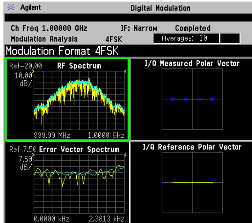
APCO25 phase1 Error Vector Spectrum (Quad-View)
