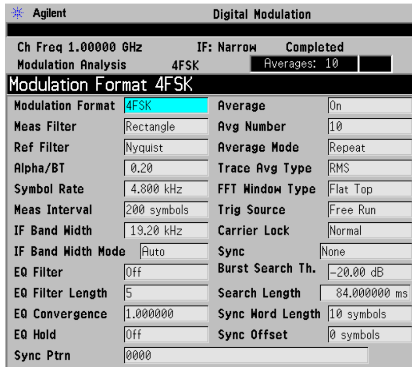
APCO25 phase1 Meas Setup Table Example
