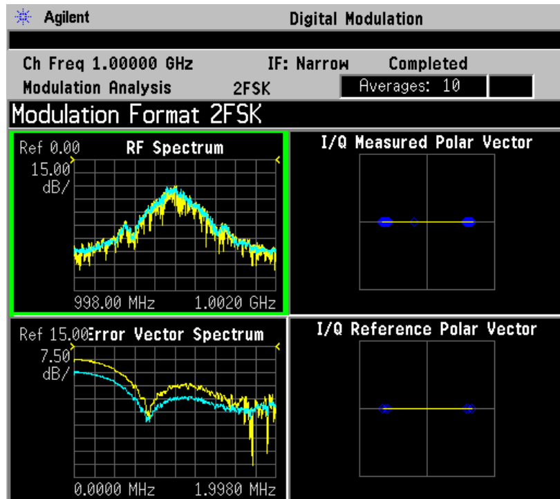
Bluetooth Error Vector Spectrum (Quad-View)
