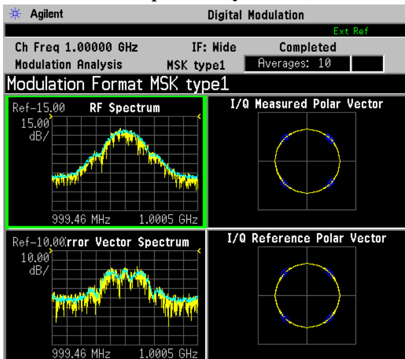
MSK Error Vector Spectrum (Quad-View)
