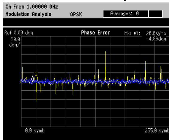
Figure 2-24 I/Q Error: Phase Error versus Symbol
